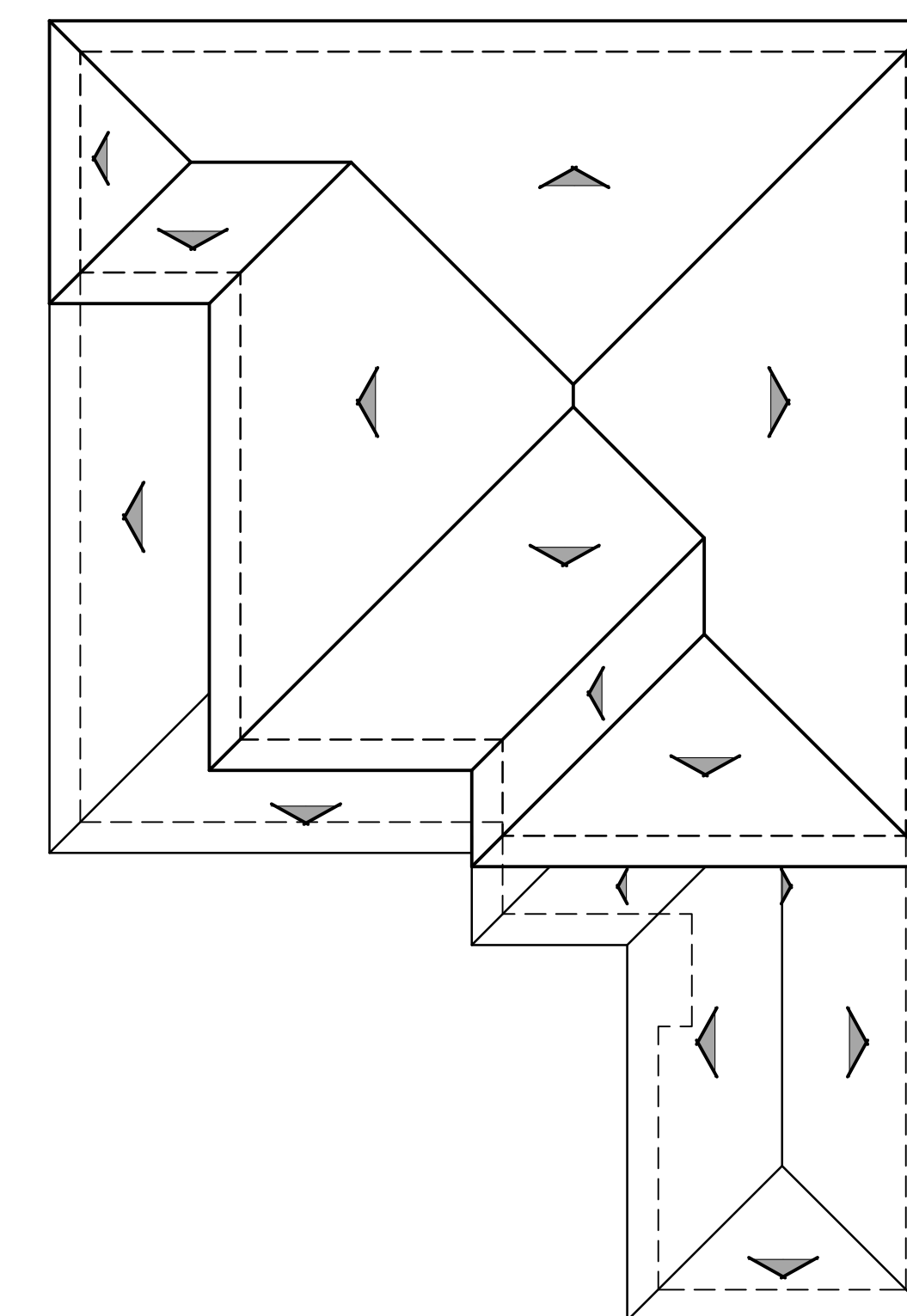
ROOF PLAN
