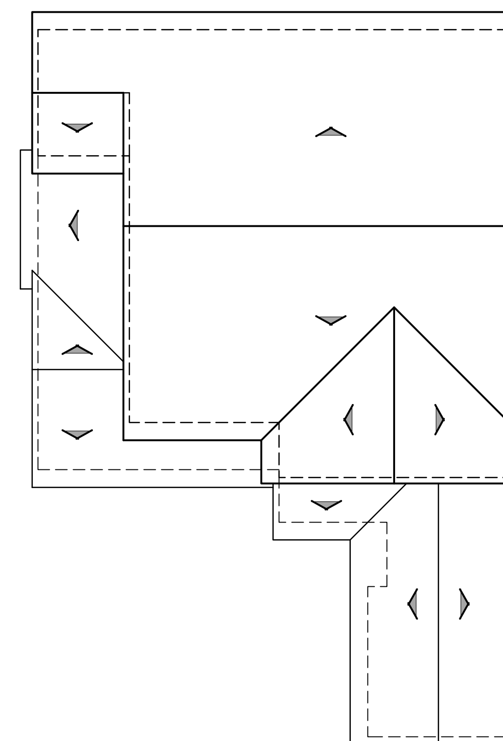
ROOF PLAN
