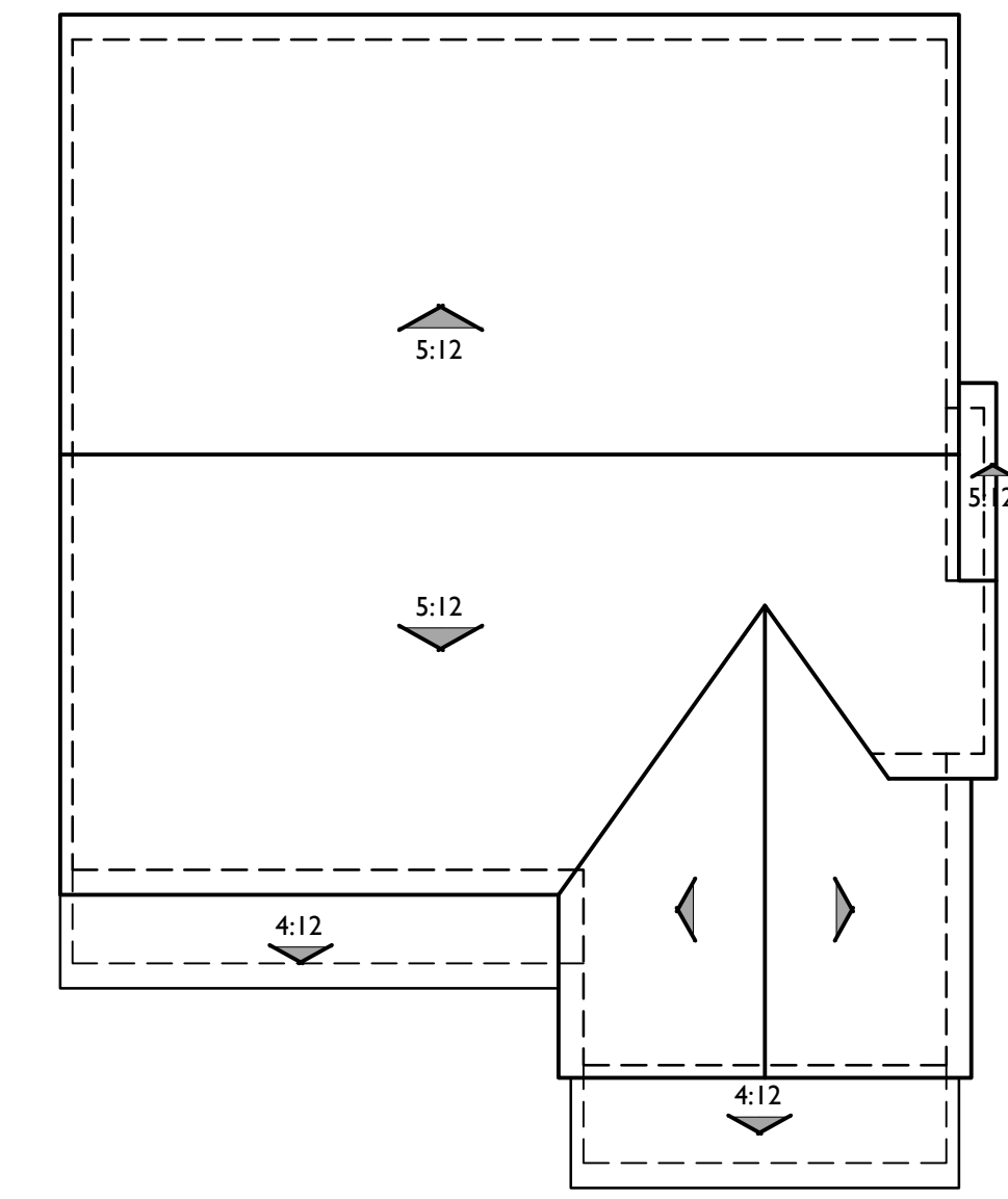
ROOF PLAN B 1/8"=1'-0" PITCH: 7:12 U.N.O. RAKE: 6" EAVE: 12" ROOF MATERIAL: CONCRETE FLAT TILE
