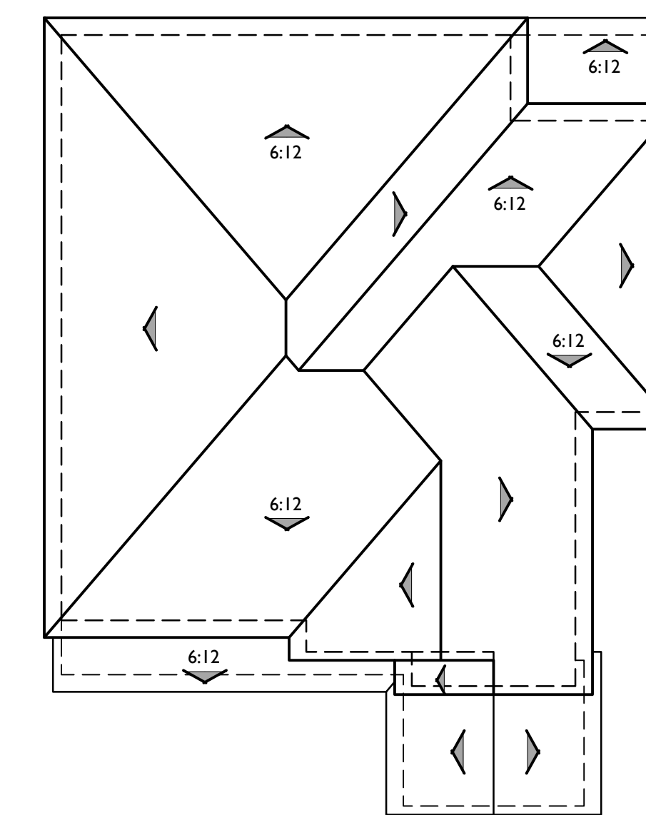
ROOF PLAN B
