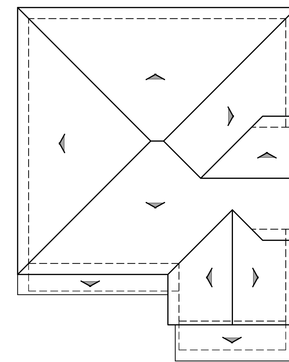
ROOF PLAN
