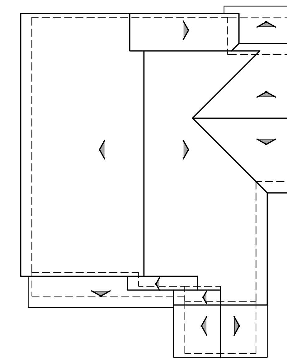
ROOF PLAN A PITCH: 3.5:12 U.N.O RAKE: 6" EAVE: 18" ROOF MATERIAL: CONCRETE 'S' TILE
