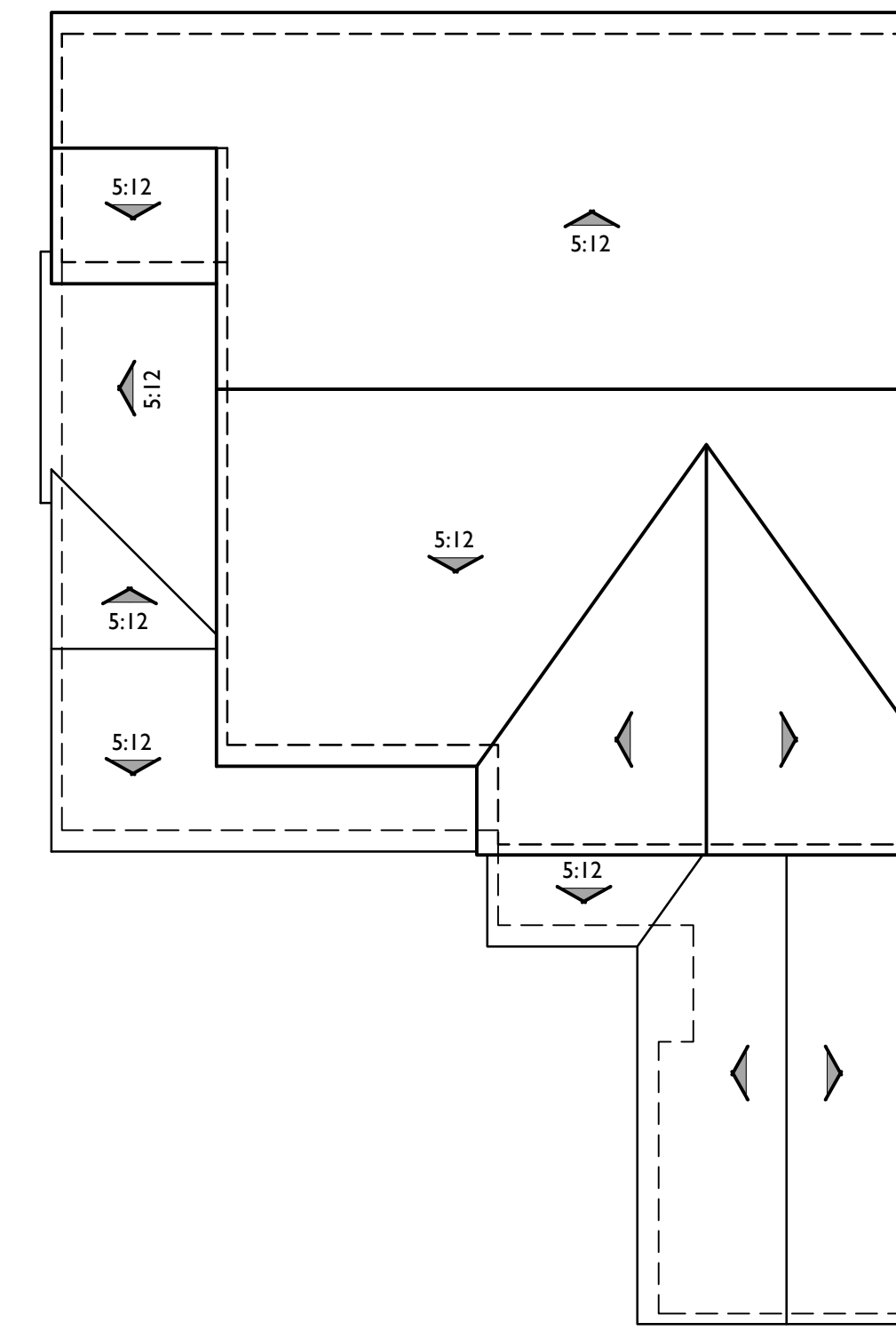
ROOF PLAN
